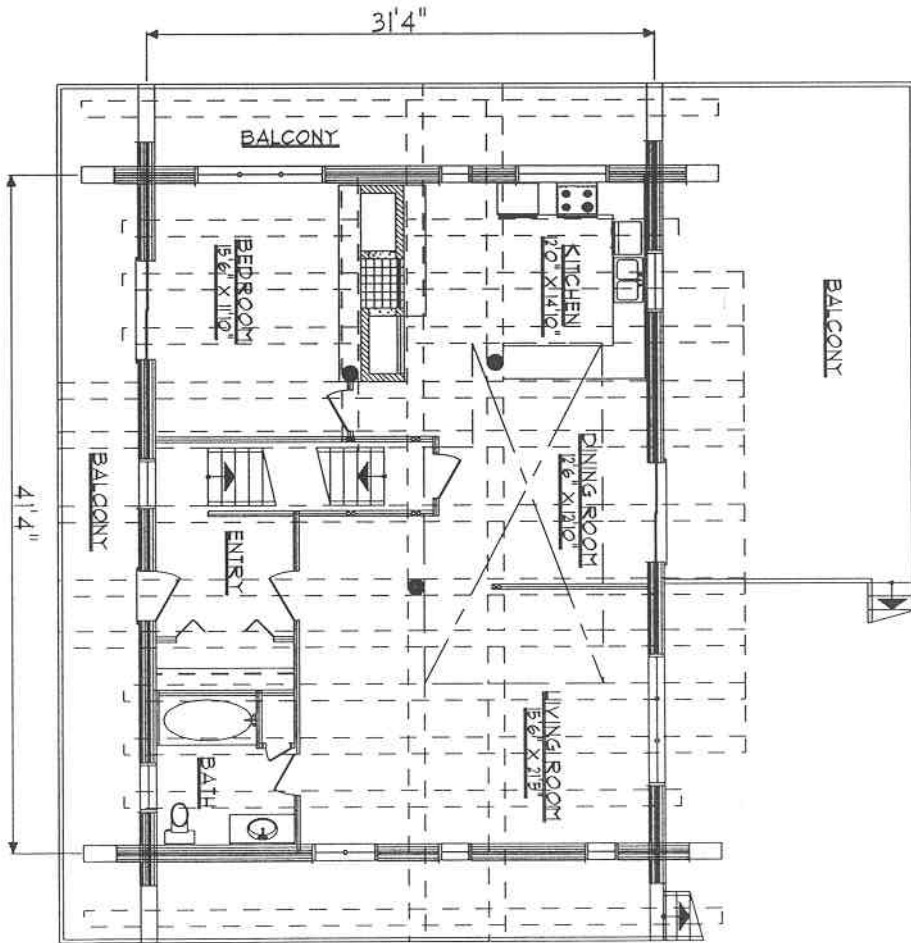
MAIN FLOOR PLAN 1344 SE
