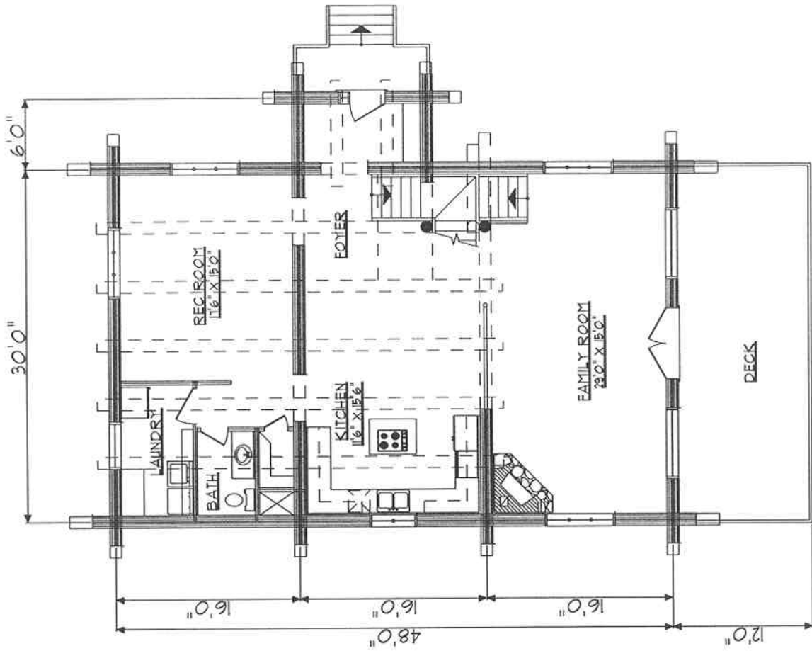
MAIN FLOOR PLAN 1556 SE
