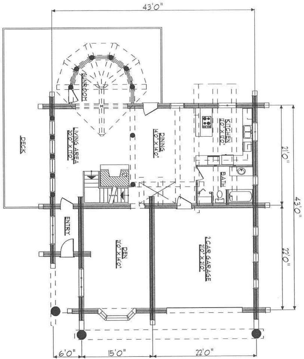
FIRST FLOOR PLAN HOUSE - 1401 SF GARAGE - 491 SF
