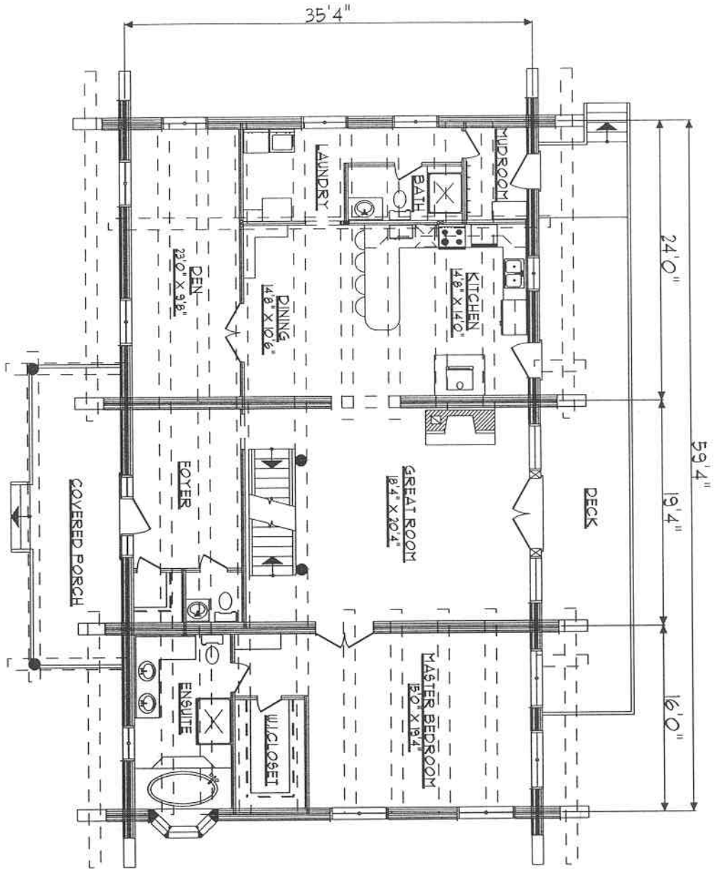
MAIN FLOOR PLAN 2160 SF
