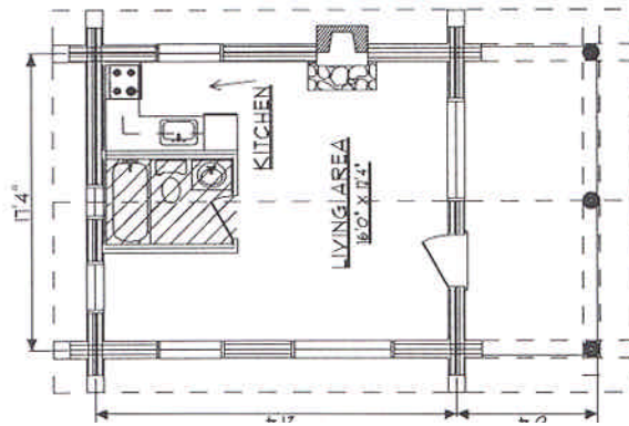
MAIN FLOOR PLAN 236 SF
